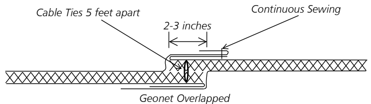
Figure 1 Overlap Along Roll Length
