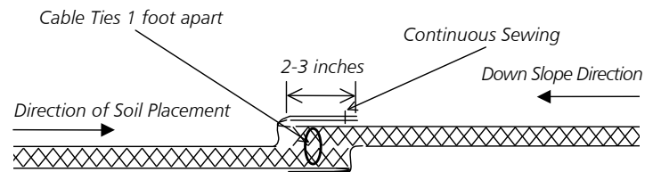
Figure 2 Overlap Along Roll Width
